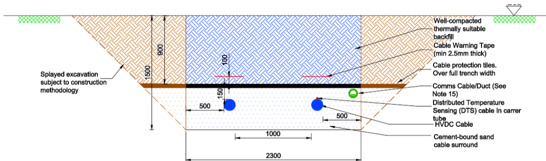
Direct Buried Cable Cross Sections - One Trench Scale 1:25
